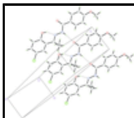
Fig. 2. Packing diagram showing intramolecular O—H···N and intermolecular N—H···O hydrogen bonds (dashed lines).
